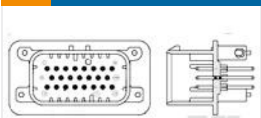
TE Part # 776200-1 23POS,PIN DIA 1.3,HDR ASSY, 180DEG,COD 1
