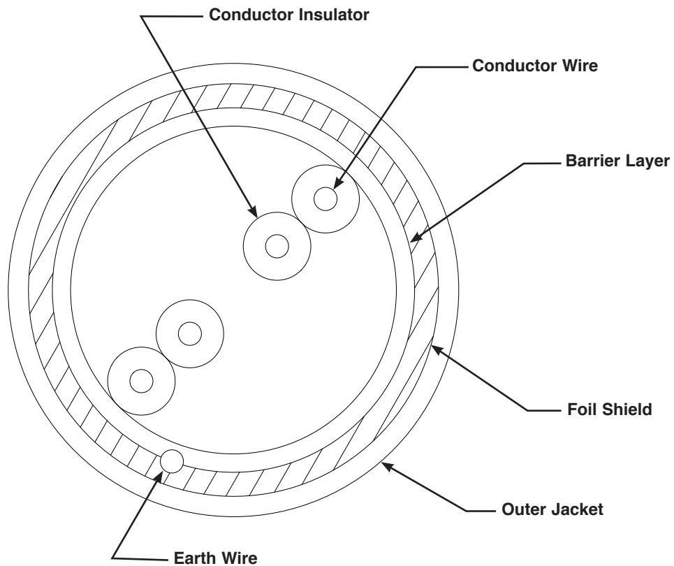
IFRH5C02BL Cable Cross-Section
