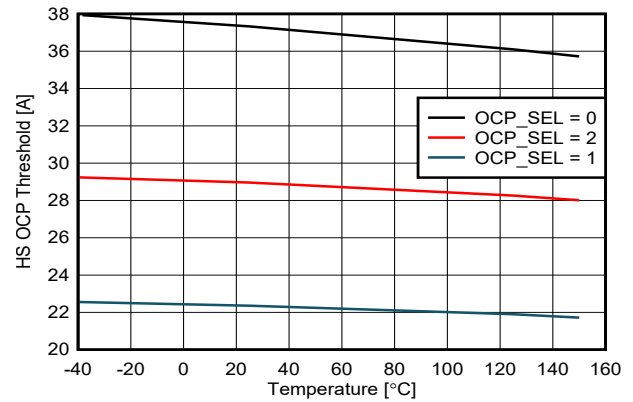
Figure 6-14. HS OCP Threshold vs Temperature at V_{VM} = 13.5 V
