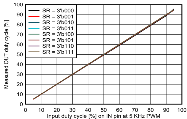
Figure 6-17. Measured Duty Cycle vs Input Duty Cycle at PWM frequency of 5 KHz at V_{VM} = 13.5 V for HS recirculation
