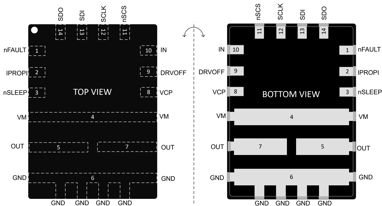
Figure 5-4. DRV8143S-Q1 SPI(S) variant in VQFN-HR (14) package
