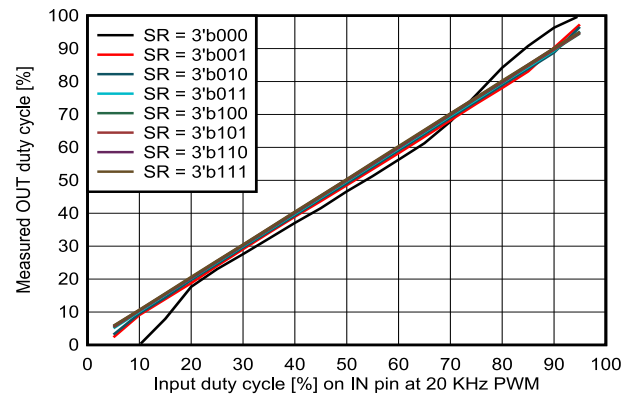
Figure 6-18. Measured Duty Cycle vs Input Duty Cycle at PWM frequency of 20 KHz at V_{VM} = 13.5 V for HS recirculation
