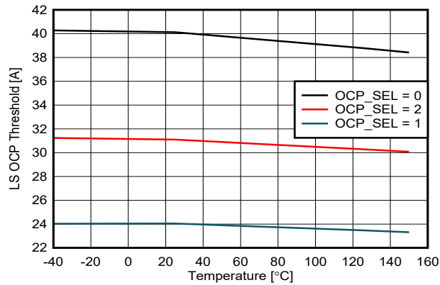
Figure 6-13. LS OCP Threshold vs Temperature at V_{VM} = 13.5 V
