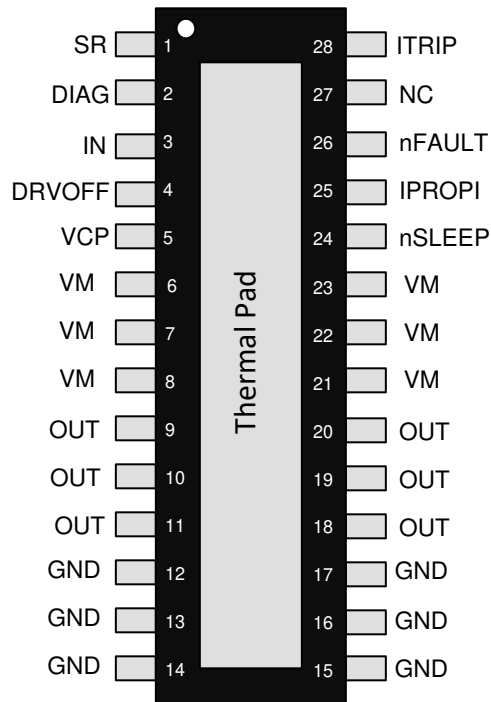
Figure 5-2. DRV8143H-Q1 HW variant in HVSSOP (28) package
