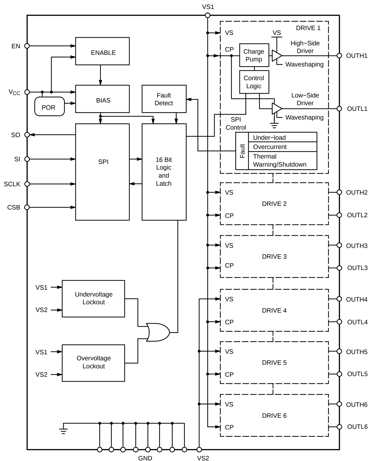
Figure 1. Block Diagram
