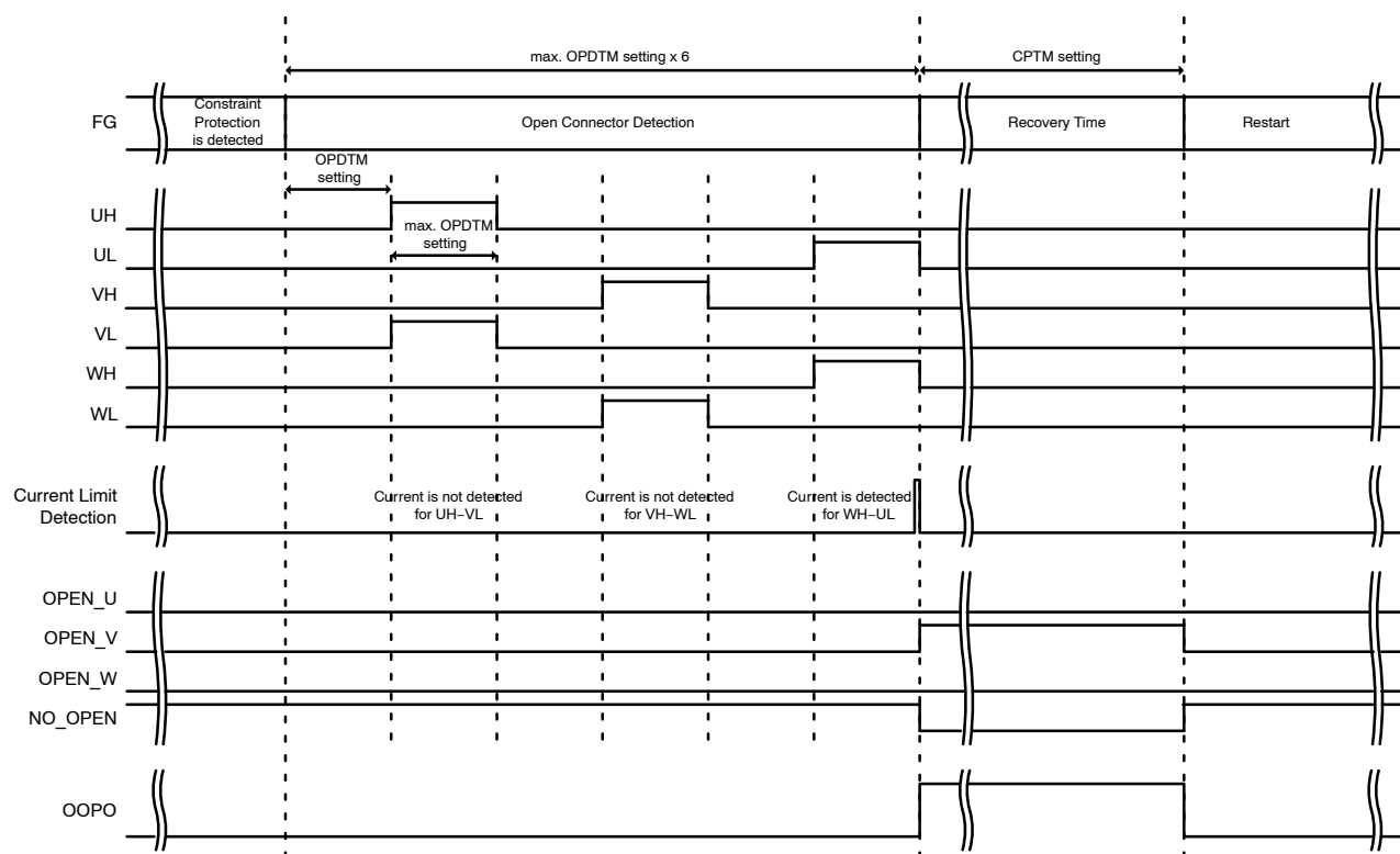
Figure 17. Timing Chart of OOPO
