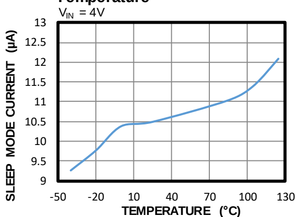
Sleep Mode Current vs. Temperature
