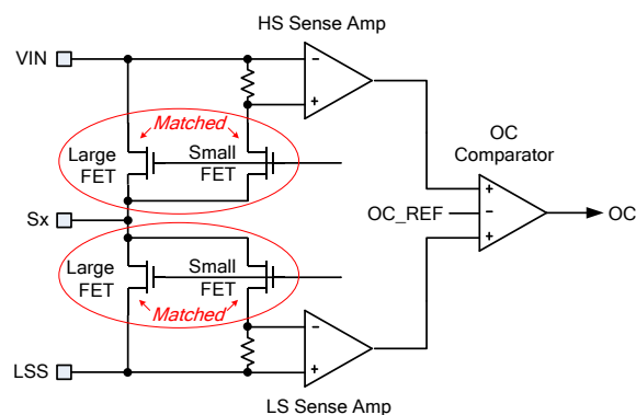
Figure 3: OCP Circuit
