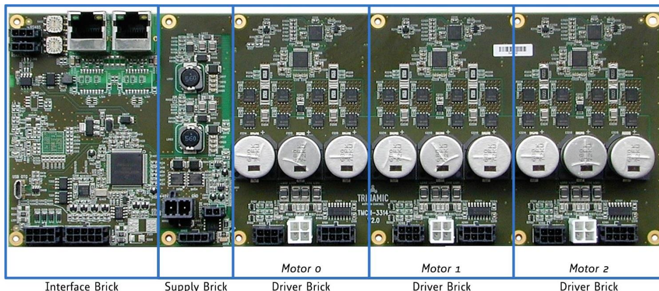
Figure 5.1 different bricks used for the TMC314 / TMC315
