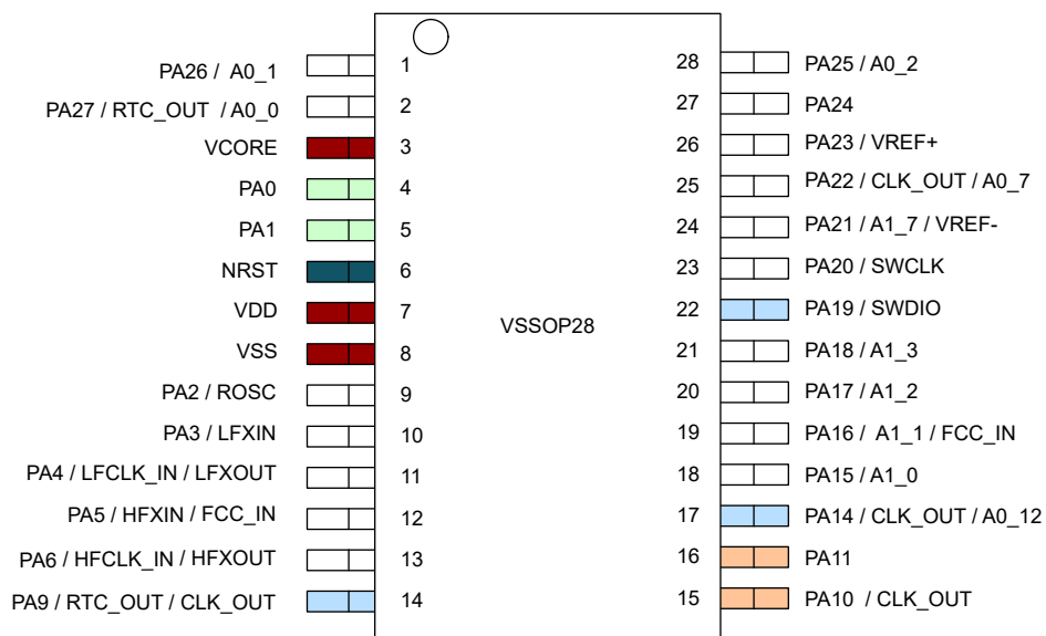
Figure 6-6. 28-Pin DGS28 (VSSOP) (Top View)
