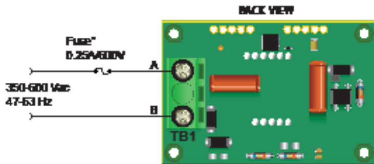
Figure 1. Wiring Diagram
