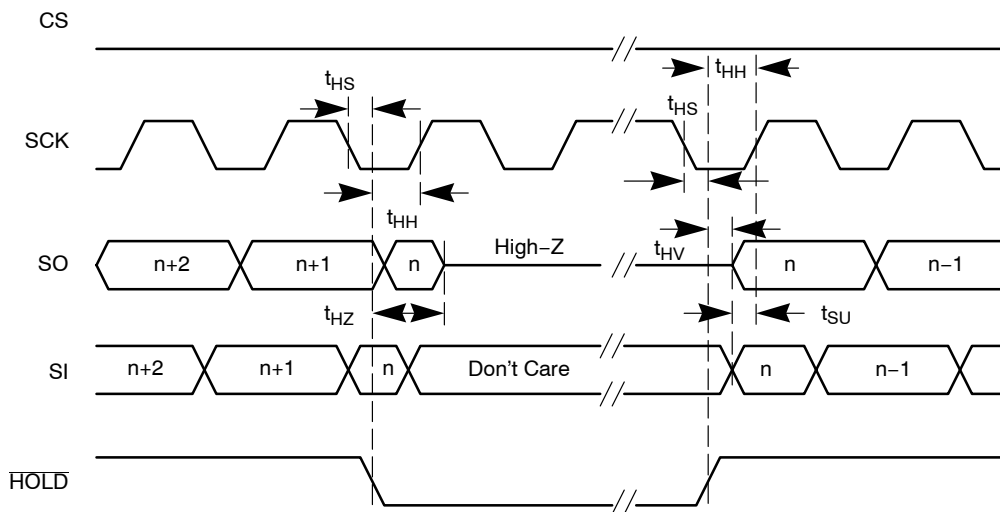
Figure 5. Hold Timing
