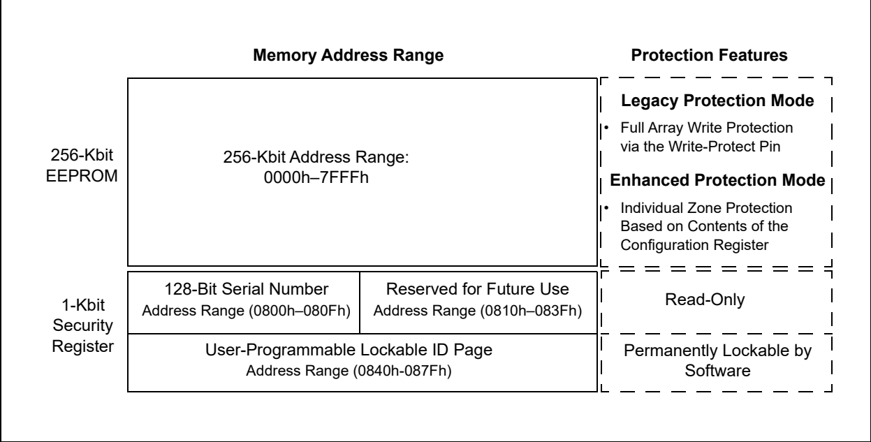
FIGURE 3-1: MEMORY ORGANIZATION
