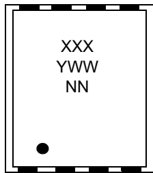
8-Lead 2x3 UDFN (Q4B)
