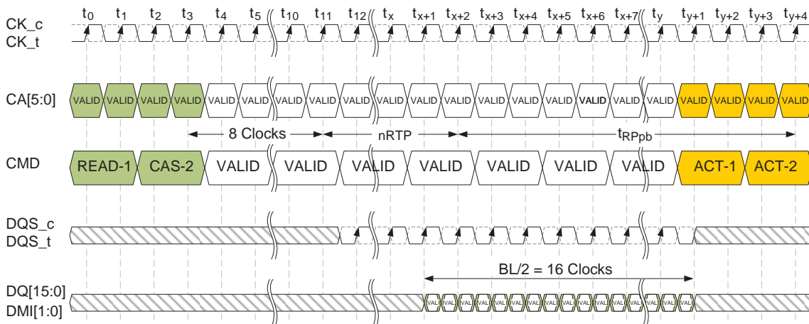
Figure 4.50 — Burst READ with Auto-PRECHARGE (Shown with BL32, 2tCK pre-ambles)
