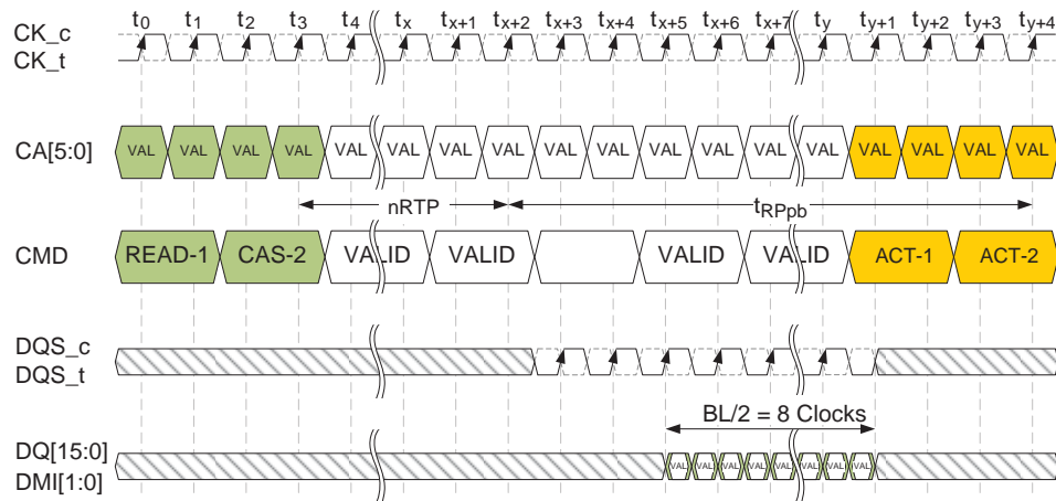
Figure 4.49 — Burst READ with Auto-PRECHARGE (Shown with BL16, 2tCK pre-ambles)
