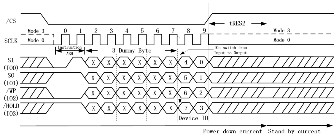
Figure 26.d. Release Power-down / Device ID Instruction (QPI Mode)
