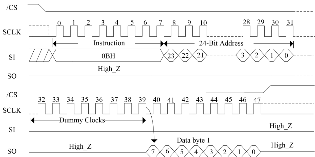
Figure 11.a. Fast Read Sequence Diagram (SPI Mode)
