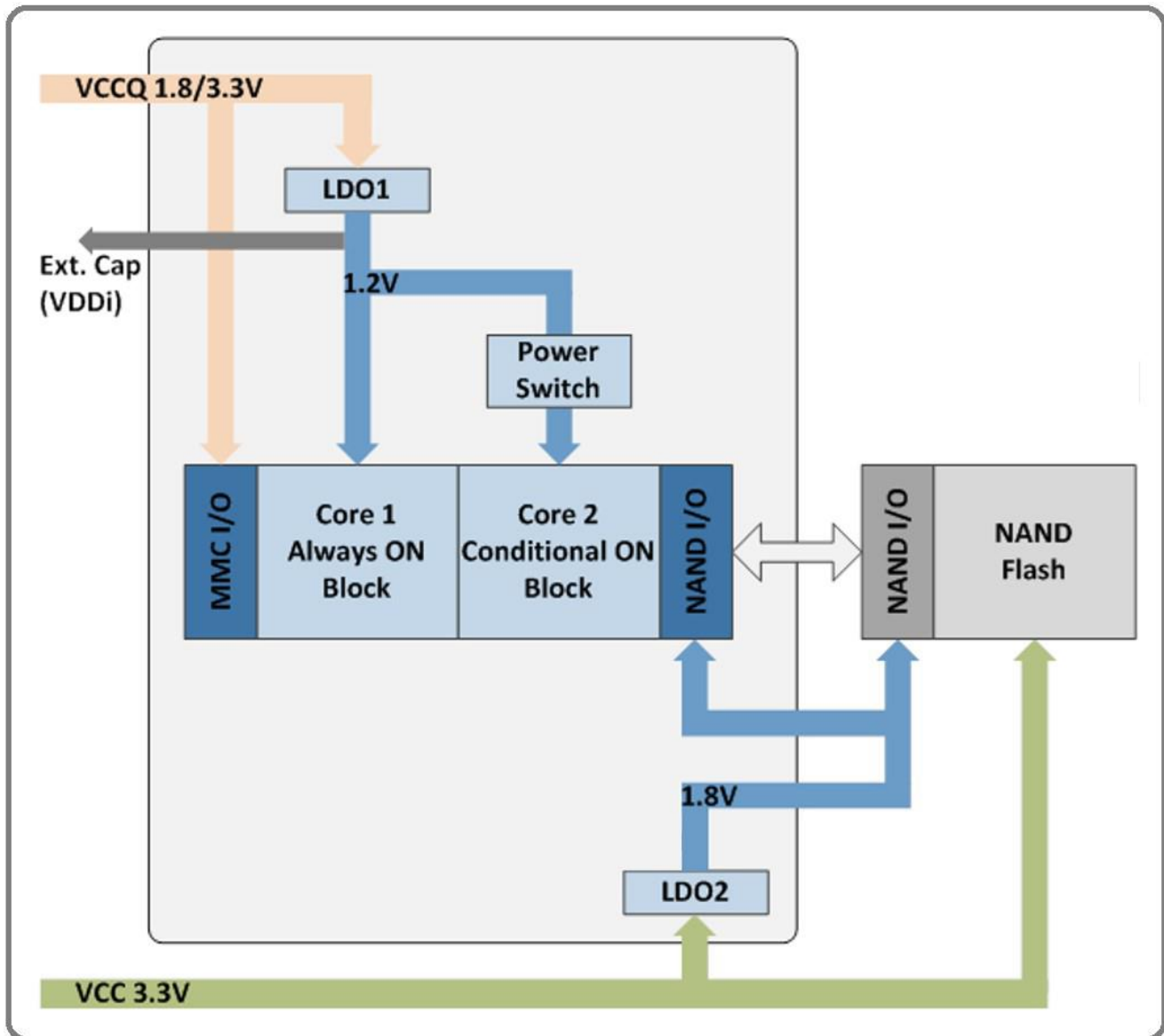
Figure 3. ASFC8G31M-51BIN Block Diagram
