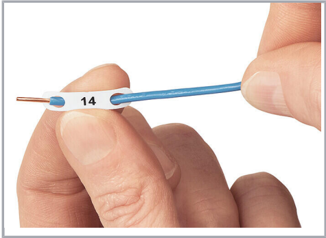
Conductor marker for thread-on mounting
