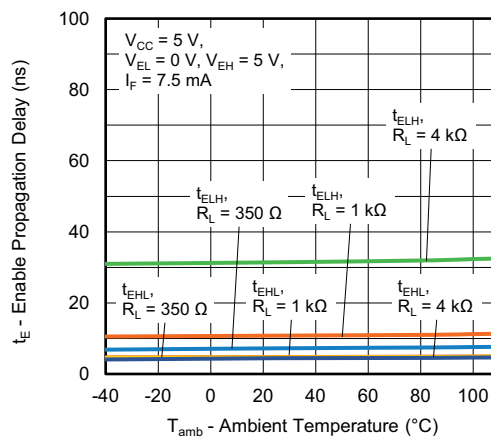
Fig. 18 - Enable Propagation Delay vs. Ambient Temperature
