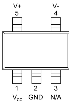
Figure 3-1. Pin Configuration (SOT23-5)
