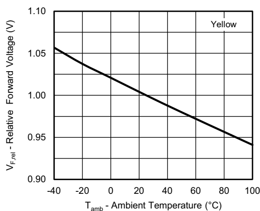
Fig. 17 - Relative Forward Voltage vs. Ambient Temperature
