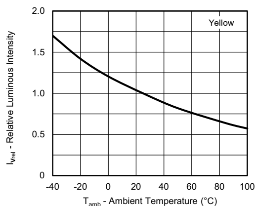
Fig. 16 - Relative Luminous Intensity vs. Ambient Temperature
