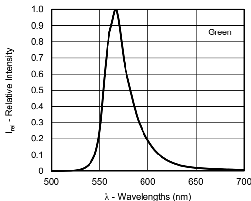
Fig. 18 - Relative Intensity vs. Wavelength
