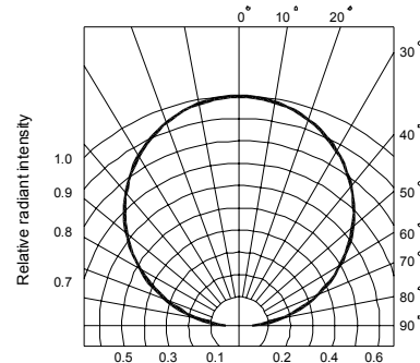
Fig.6 Radiation diagram
