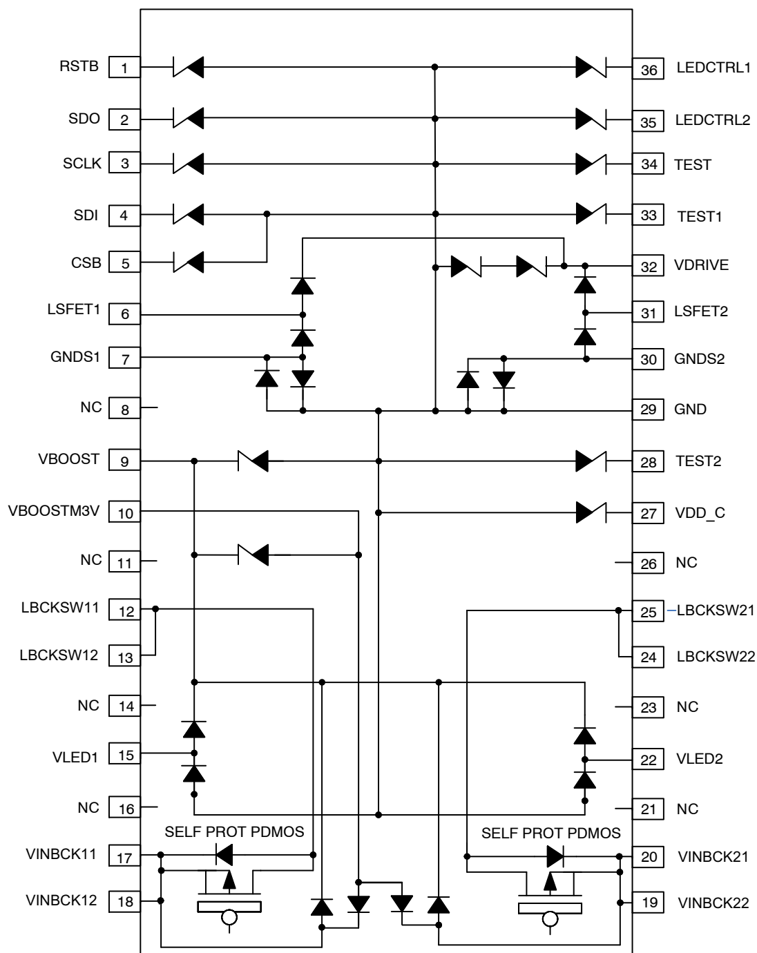
Figure 3. ESD Schematic
