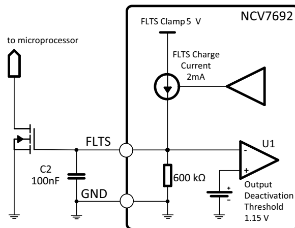
Figure 7. Open Drain Output Interface to Microprocessor
