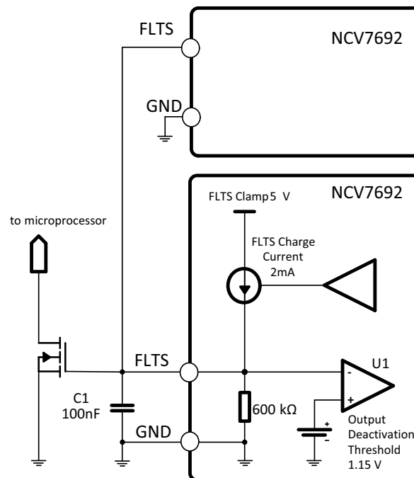
Figure 8. FLTS Wired OR to Microprocessor
