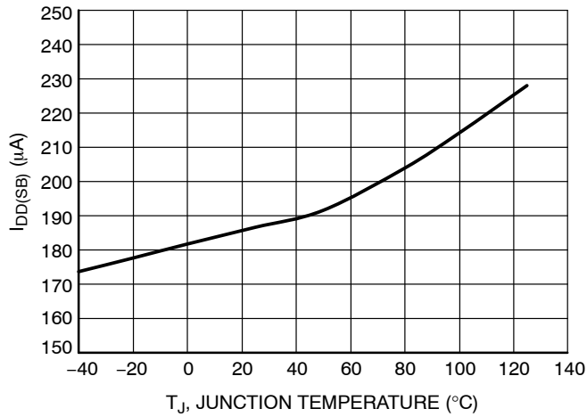
Figure 7. I DD(SB) vs. Temperature
