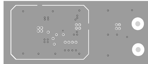
Mid-Layer 1
