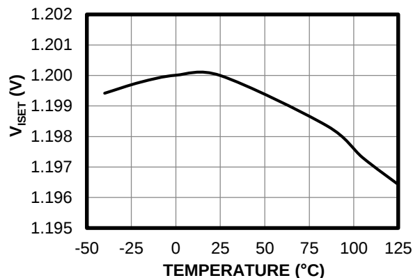
ISSET Voltage vs. Temperature
