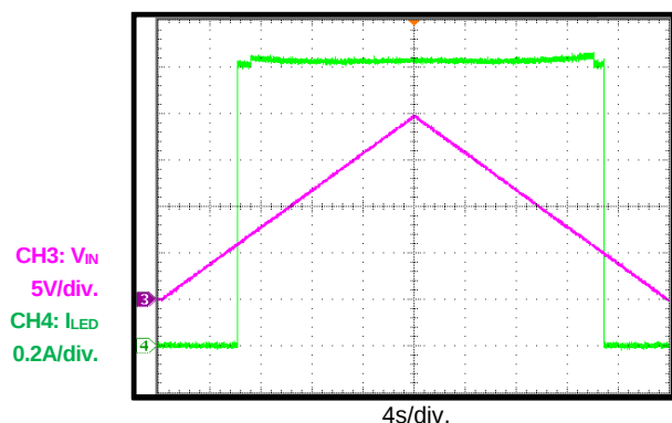
V_{IN} Slow Ramp Up and Down
