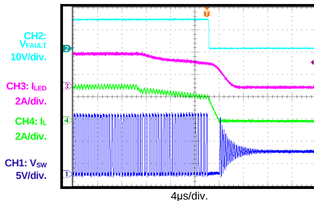
ISSET Open Fault after IC Starts Up
