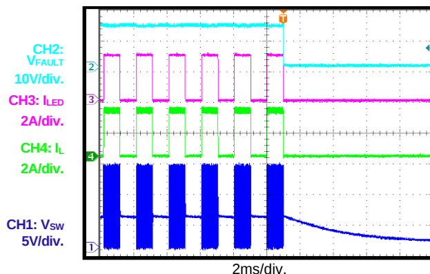
ISSET Open Fault after IC Starts Up PWM dimming
