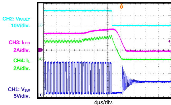
ISSET Short Fault after IC Starts Up
