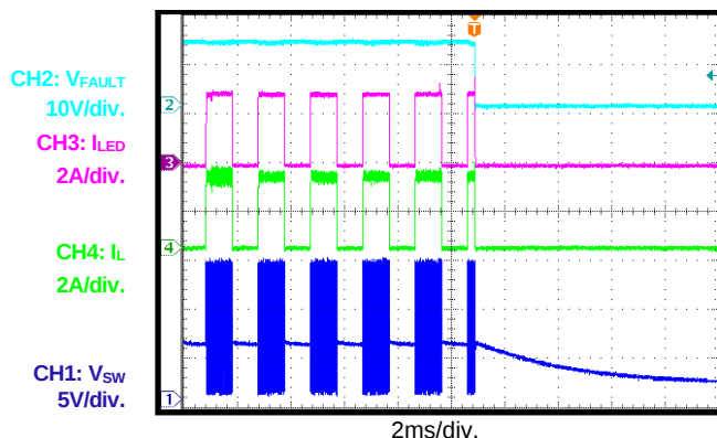
ISSET Short Fault after IC Starts Up PWM dimming
