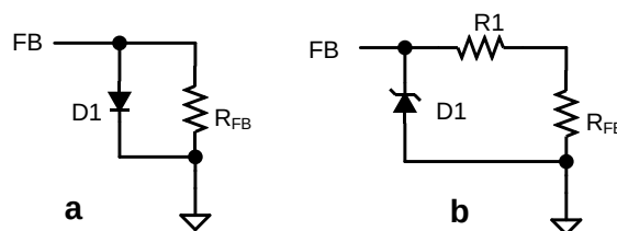
Figure 3: Short Load Protection on the FB Pin
