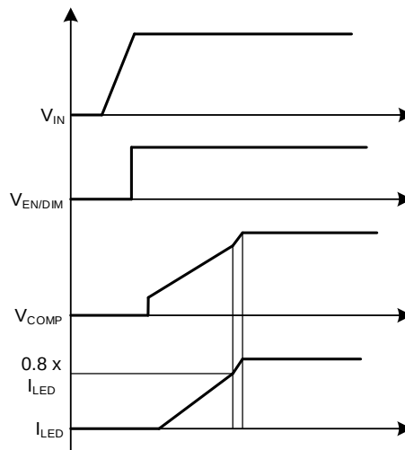
Figure 2: Soft-Start Process
