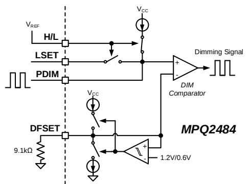
Figure 12: PWM Dimming
