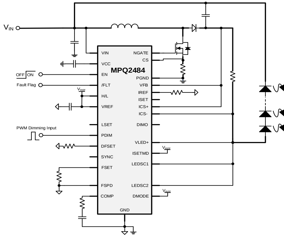
Figure 2: Buck-Boost Configuration
