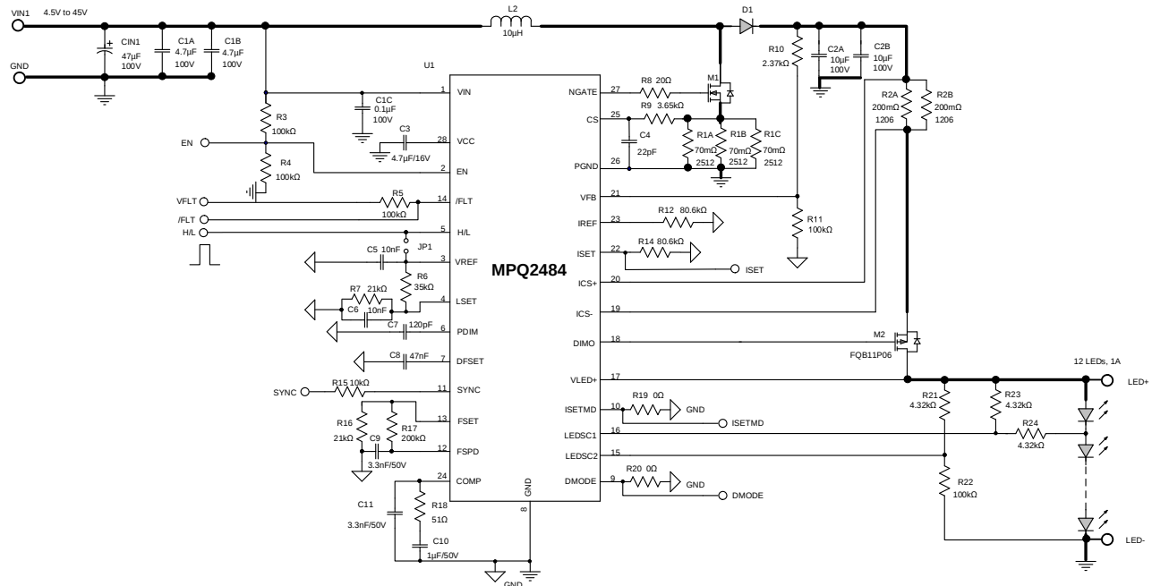
Figure 17: Typical Application Circuit for Boost Topology (Two-Step Dimming)
