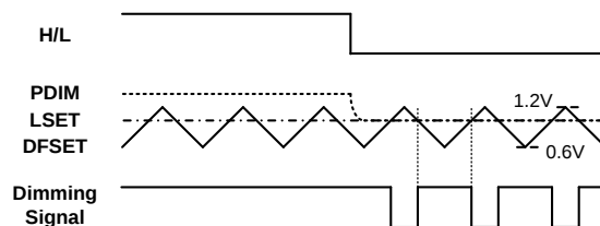
Figure 11: Dimming Signal Generation
