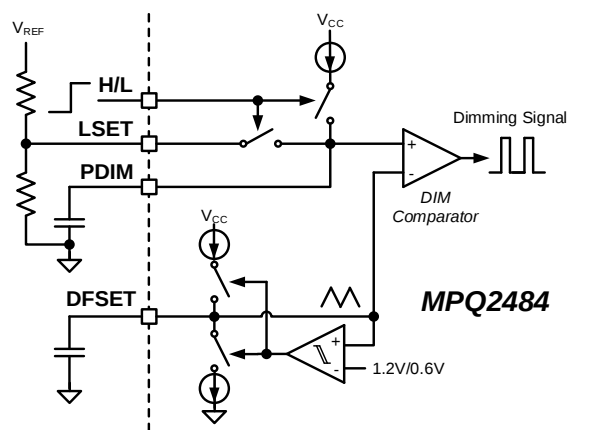
Figure 7: Two-Step Dimming
