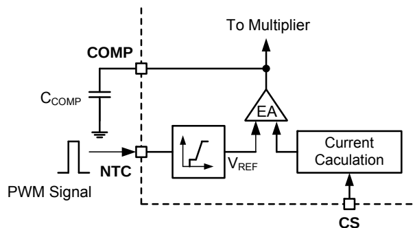
Figure 12: PWM Dimming
