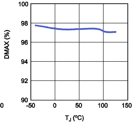
Maximum Duty vs. T_J R_T=499k\Omega
