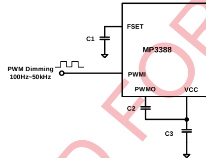
Figure 3—PWM Dimming
