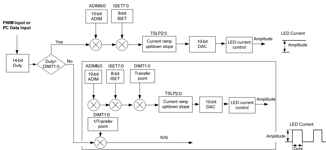
Figure 4: Mix Dimming Mode Flow Chart
