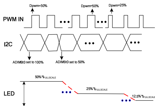
Figure 5: Analog Dimming from PWM Input
