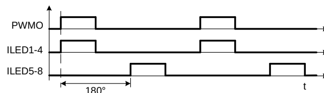
Figure 19: Phase Shift with 2 Channels
