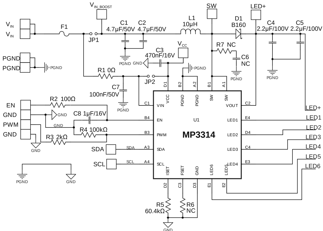
Figure 12: Typical Application Circuit
