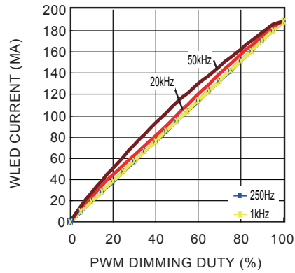
PWM Dimming Duty vs. WLED Current
