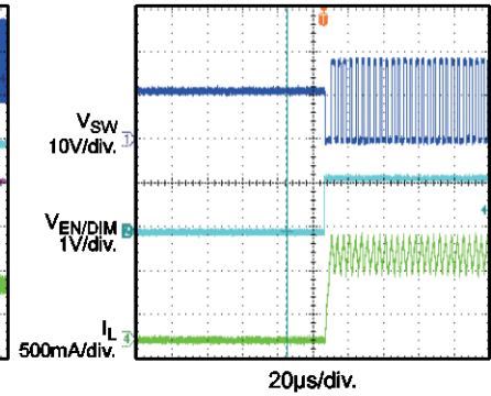
VEN Start-Up
