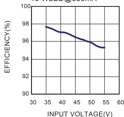
Efficiency vs. Input Voltage 10 WLED@330mA
