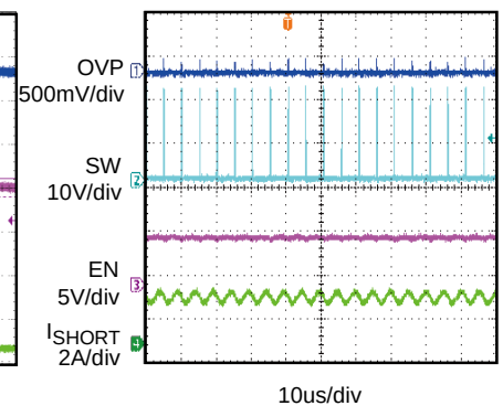
Short Circuit Protection (short LED + to VSS)
