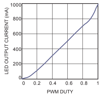
PWM Dimming
