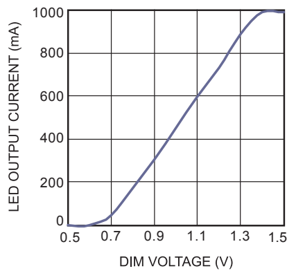
Analog Dimming
