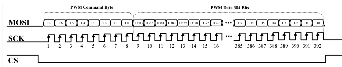
Figure 4 SPI Writing PWM Register Data to IS32FL3749
