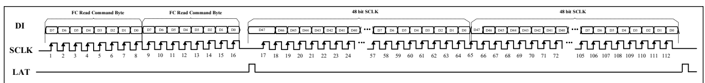
Figure 19 VSB Reading from IS32FL3749 (Two Chips Cascade, Bi-direction, read data from DI)
