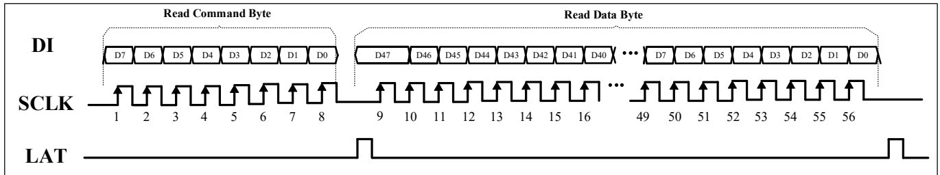
Figure 16 VSB Reading from IS32FL3749 (Bi-direction, read data from DI)
