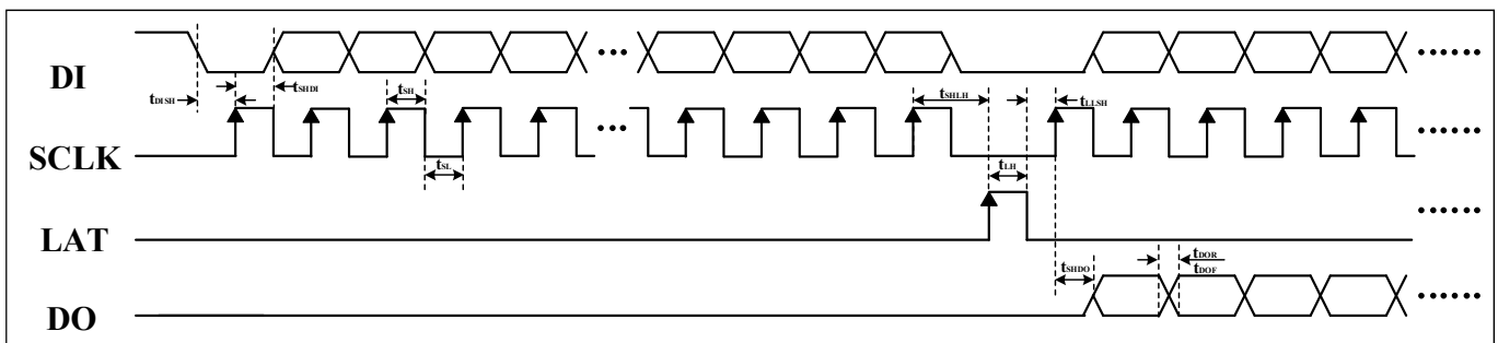
Figure 11 IS32FL3749 VSB Input Timing
