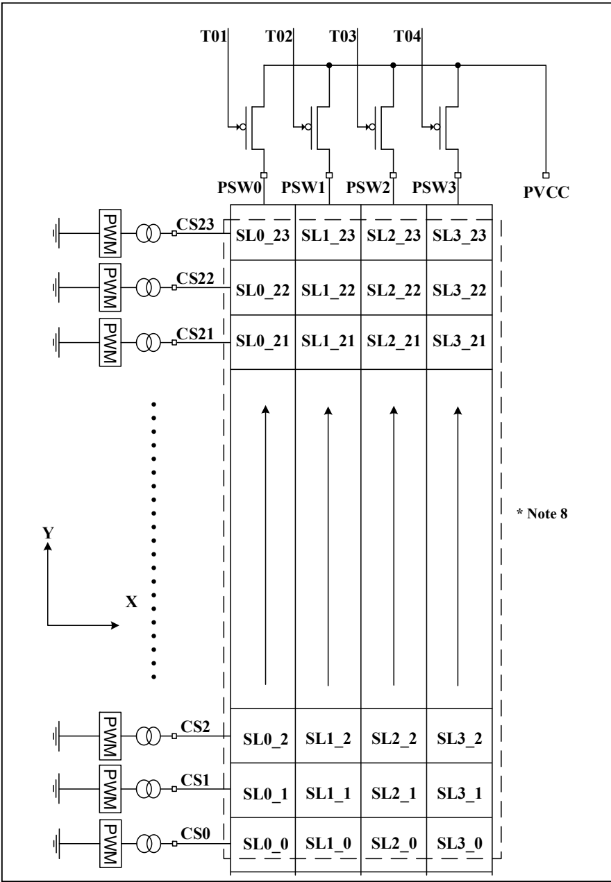
Figure 22 SL Register
