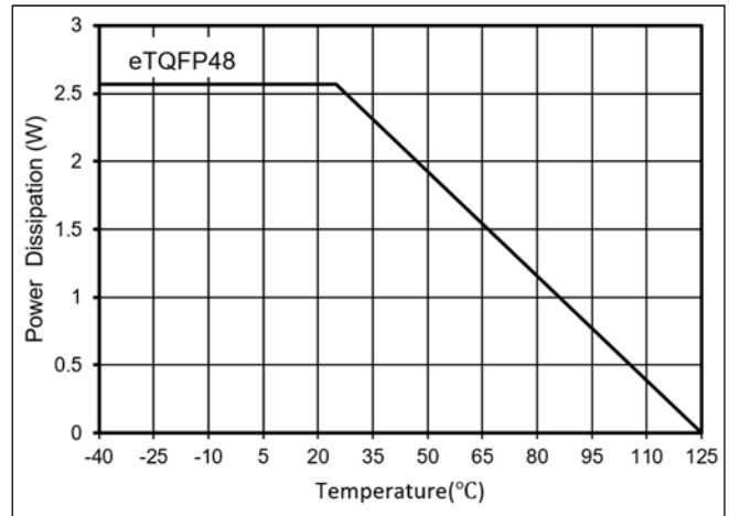
Figure 27 Dissipation Curve
