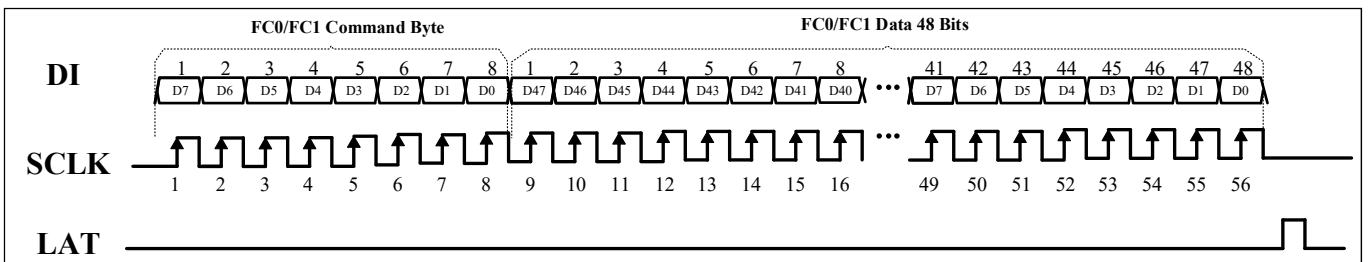
Figure 14 VSB Writing FCx Register Data to IS32FL3749
