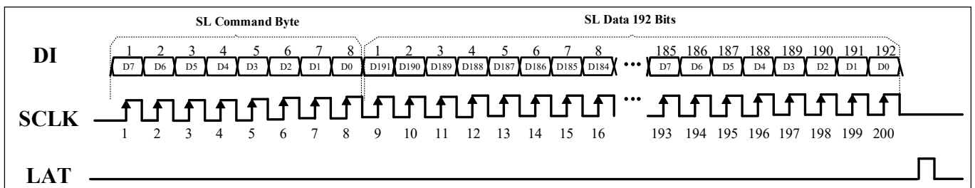
Figure 13 VSB Writing SL Register Data to IS32FL3749
