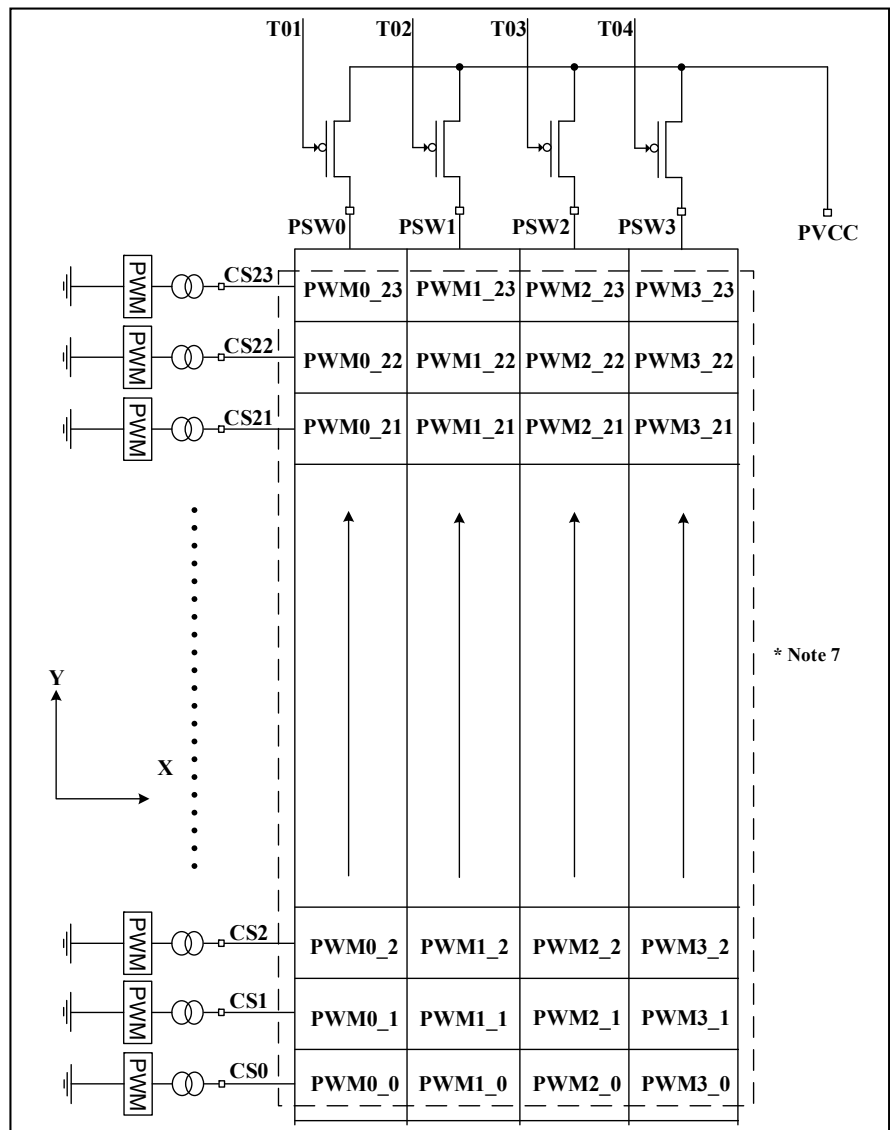
Figure 21 PWM Register
