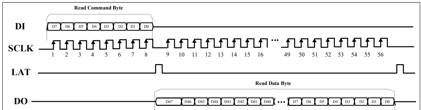
Figure 17 VSB Reading from IS32FL3749 (Single-direction, read data from DO)
