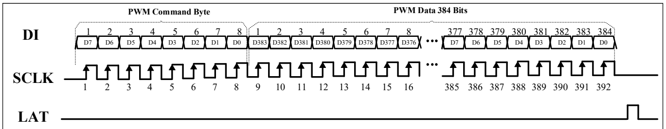
Figure 12 VSB Writing PWM Register Data to IS32FL3749
