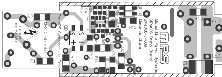
Figure 3 - Bottom Layer
