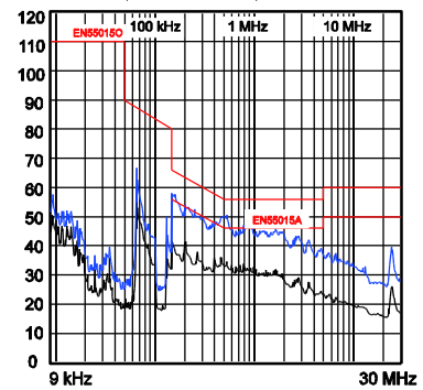
Conduction EMI
