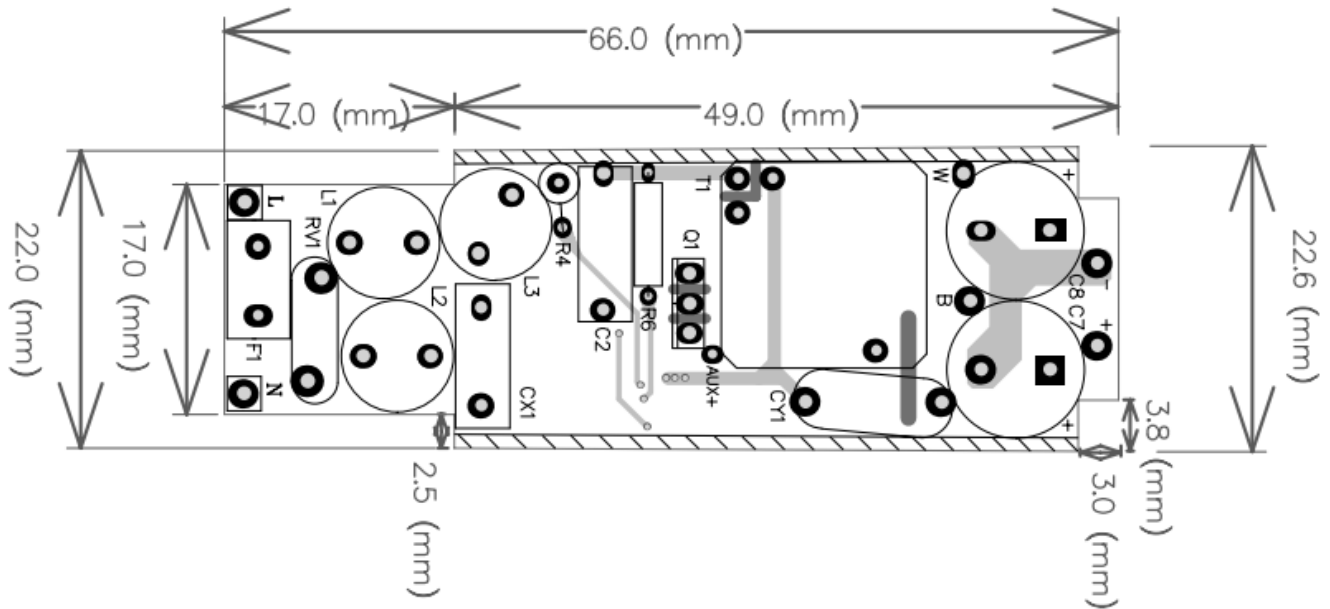
Figure 2 - Top Layer
