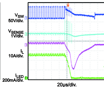
Short-Diode Protection
