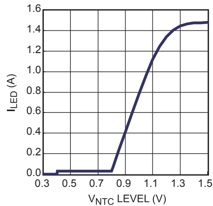
NTC Curve
