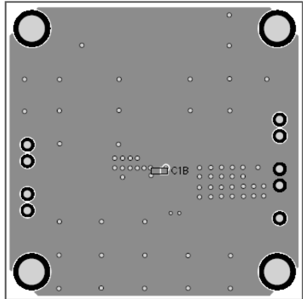
Figure 3 - Bottom Layer
