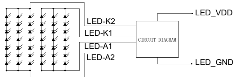
Backlight Circuit
