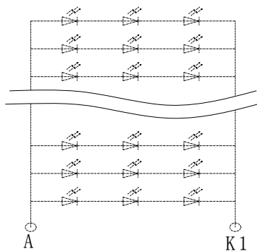
Serial line 3 and 9 27LED
