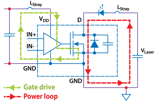
Figure 10: Recommended Layout
