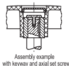
Assembly example with keyway and axial set screw
