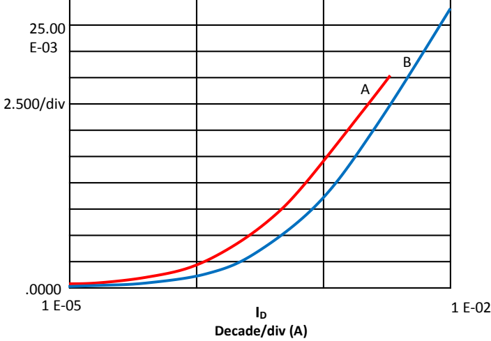
Common Source Transconductance vs. Drain Current LSK170A & B - G_{FS} vs. I_D
