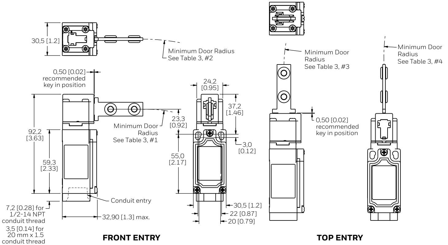
Figure 3. Product Dimensions mm [in]
