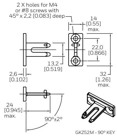
Figure 5. GKZ52M Key Dimensions
