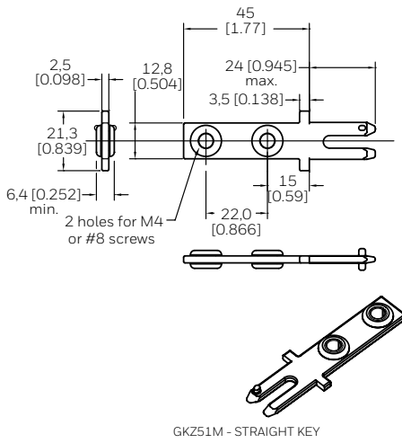
Figure 4. GKZ51M Key Dimensions
