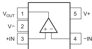
Figure 5-1. TLV365-Q1 DBV Package, 5-Pin SOT-23 (Top View)
