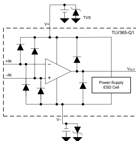
Figure 7-2. ESD Protection Scheme
