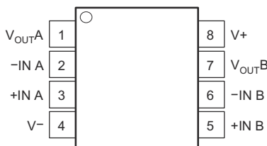
Figure 5-2. TLV2365-Q1 D (Preview) Package, 8-Pin SOIC (Top View)
