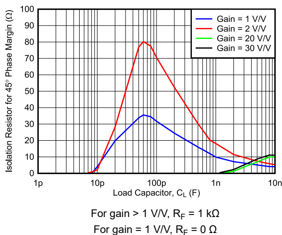
Figure 7-5. Recommended Isolation Resistor vs Capacitive Load
